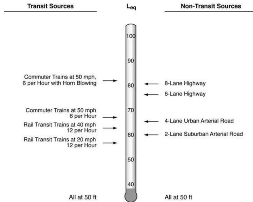
Figure B-9 Typical Hourly L_{eq}(1 \text{ Hr}) 's
